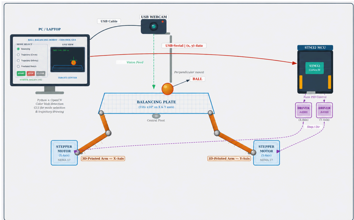
Functional Diagram
